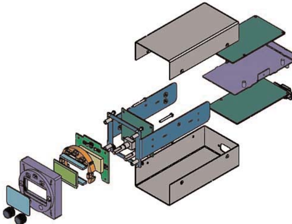
Exploded View of the radio's assembly components
