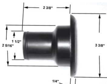
Side view of fill fitting with measurements
