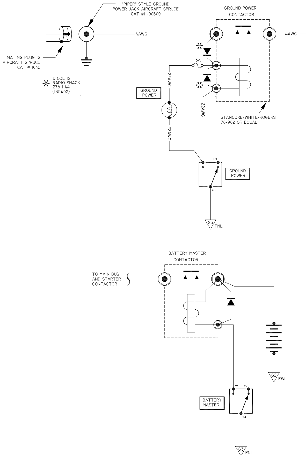
Figure 4. Gnd Pwr Control without OV Protection
