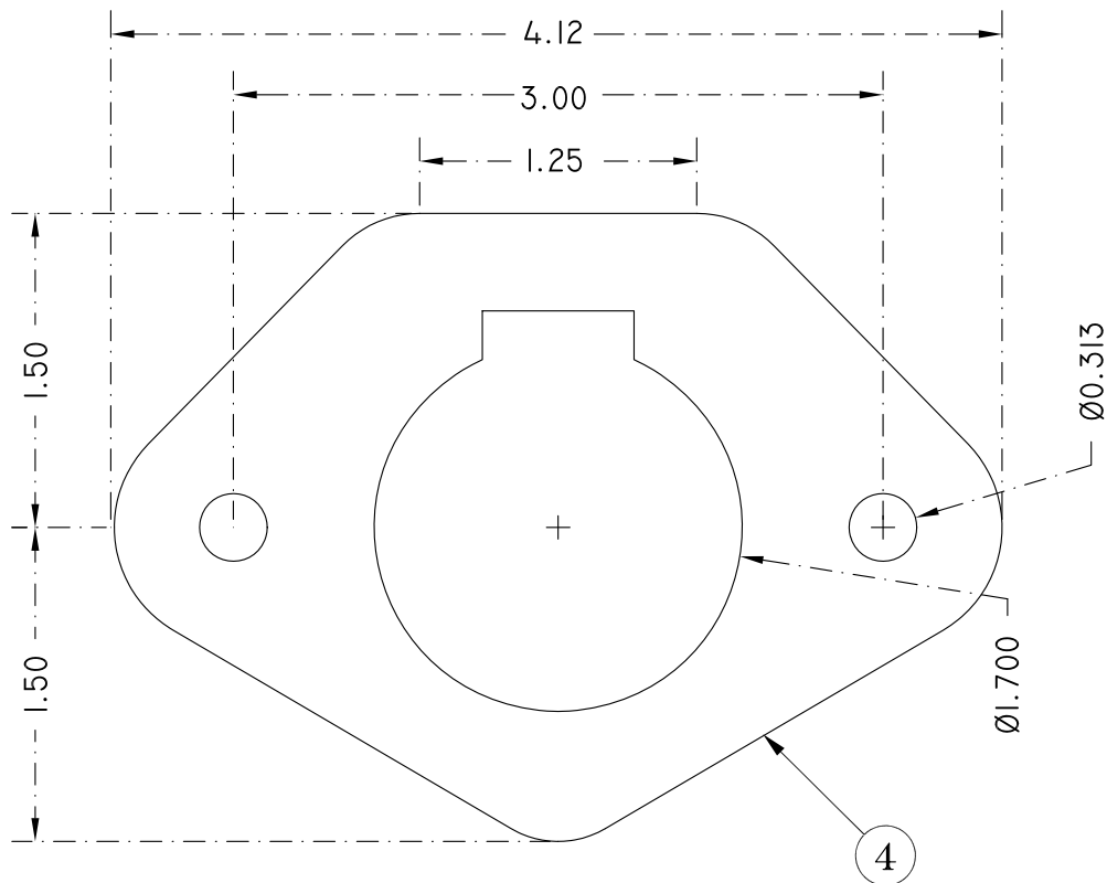
Figure 1. Brass Backplate Fabrication
