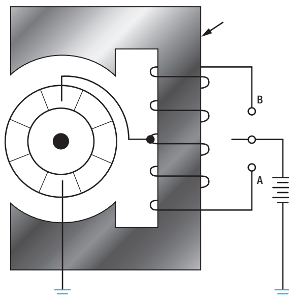
Figure 12-33. Split field series motor.
