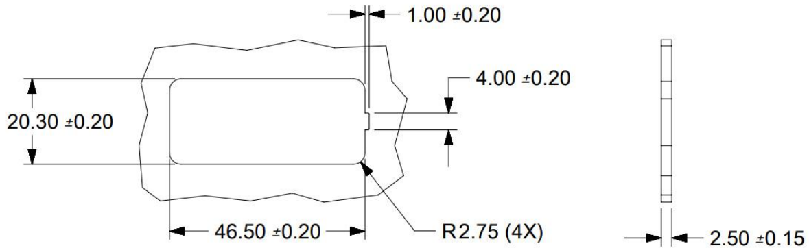
RECOMMENDED PANEL OPENING
