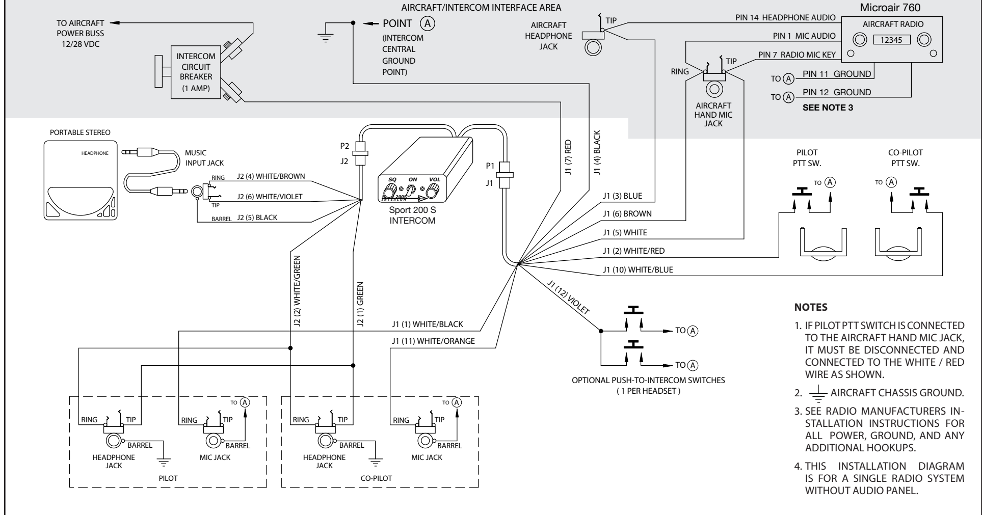
Sport 200S – Microair 760 Radio Installation Wiring Diagram
