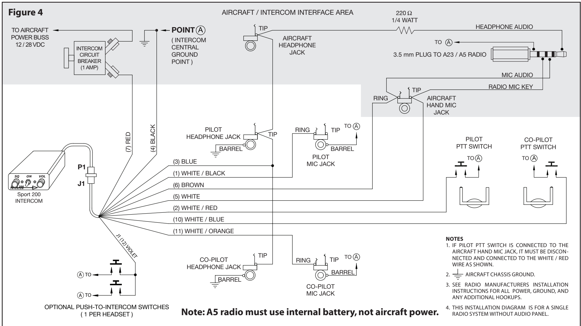
Sport 200 – ICOM A23, A5 Radio Installation Wiring Diagram
