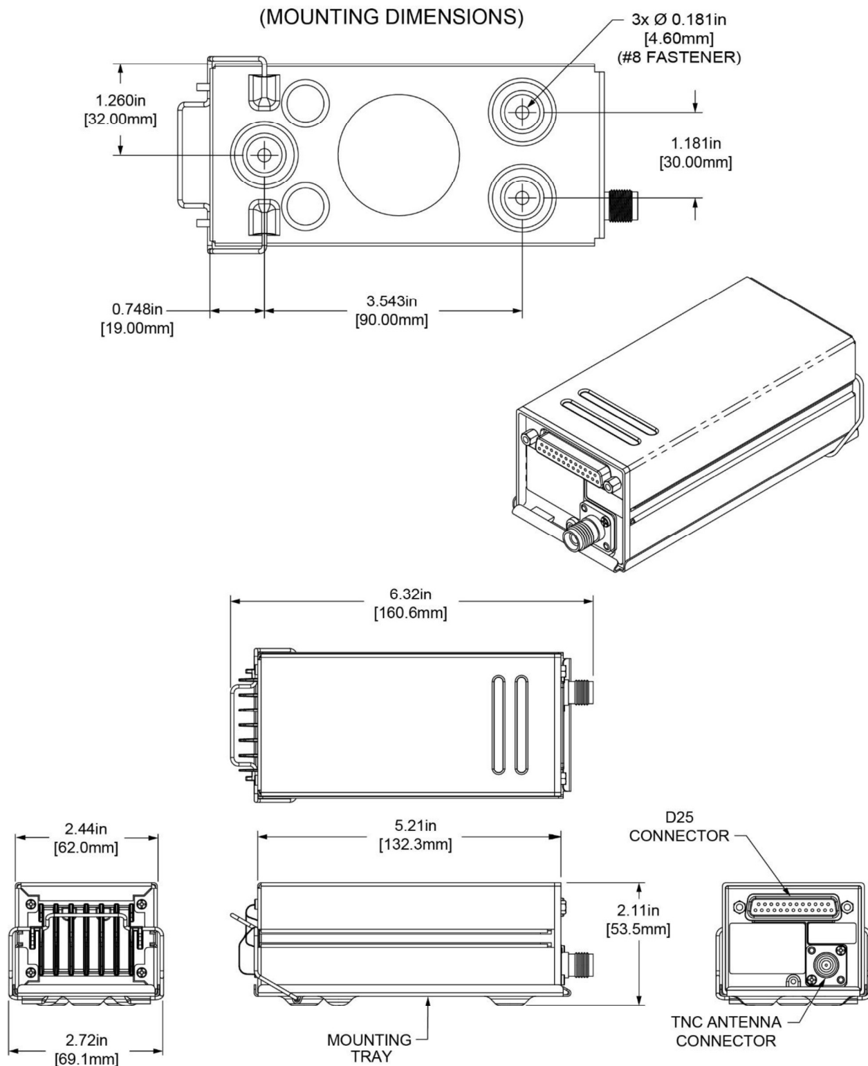
Figure 199 – SV-COM-T25/T8 Mounting Dimensions
