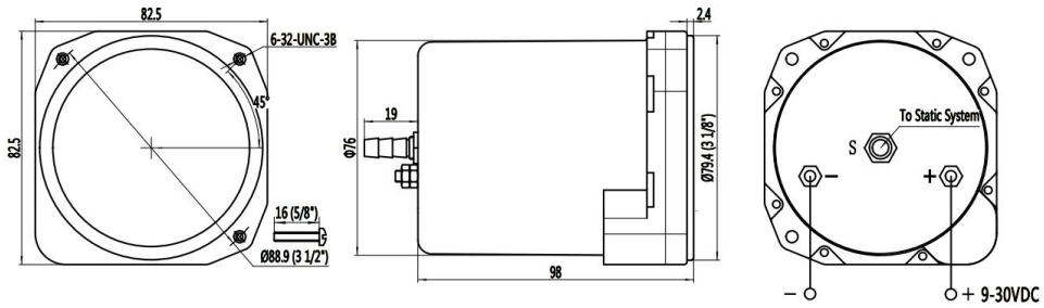
Vertical speed indicator scale drawing
