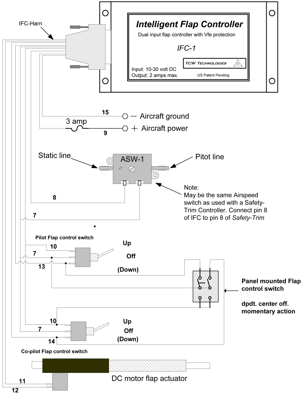
Wiring Diagram Model IFC-1
