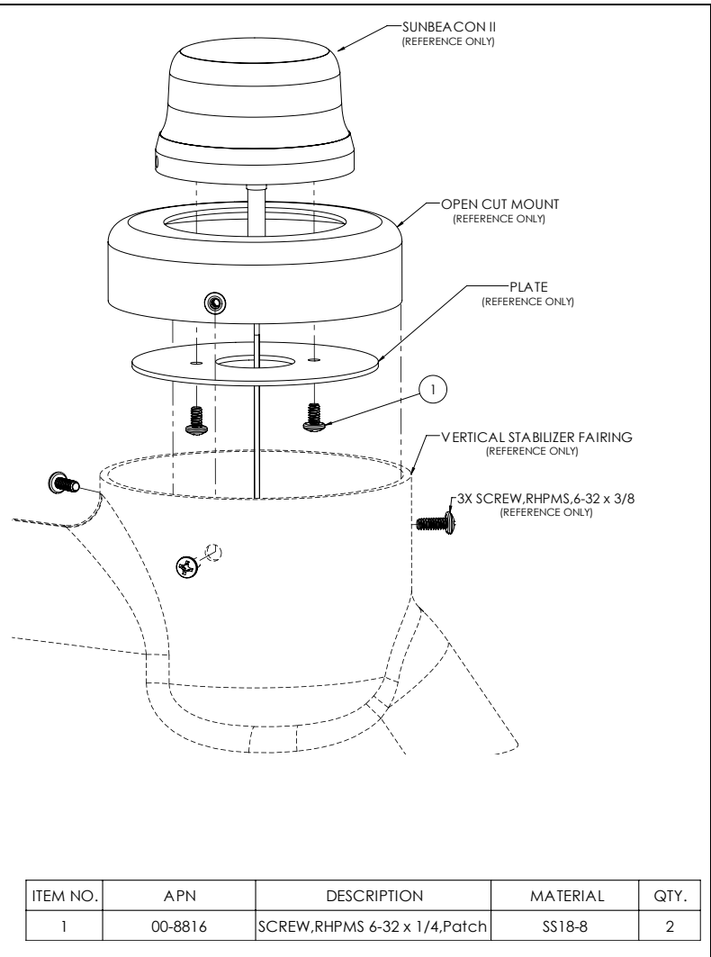
Config D: Plate Mount
