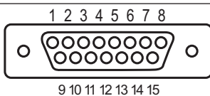
DB15 FEMALE plug viewed from the rear (wire) side
