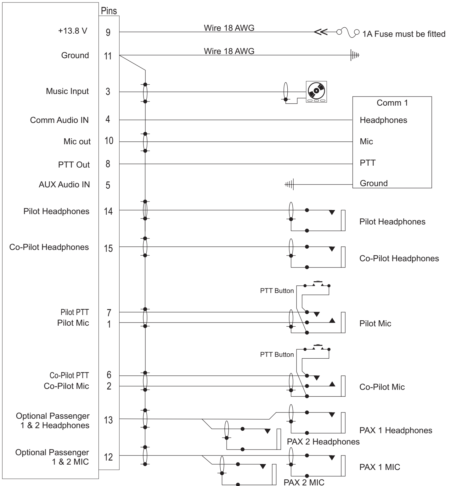
DB15 FEMALE plug viewed from the rear (wire) side
