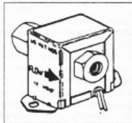
Figure #5 - Facet makes an excellent solid state fuel pump. Uses 12 volts DC power to produce a constant 5.8 psi.
