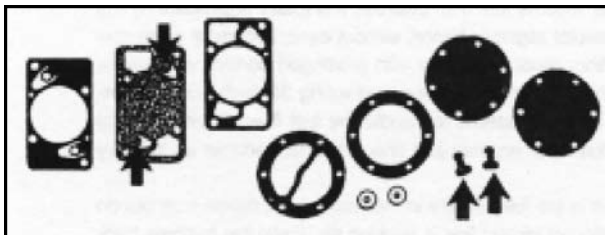
Figure #3 - Fuel pump repair kits can zero time any Mikuni Fuel Pump. Arrow shows flapper valves that causes the fuel to flow in one direction only. As simple as it gets yet surprisingly effective.
