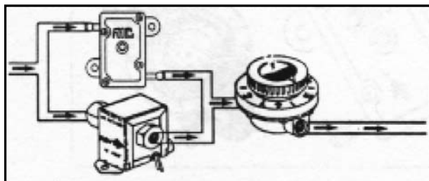
Figure #6 - Designing a redundant fuel pump system requires some special plumbing and equipment. Shown here is a parallel system that uses both electronic and pulse pumps with pressure regulator.
