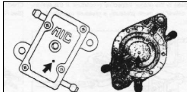
Figure #4 - The “weep hole” is located as shown by the arrow. This hole allows for fuel from engine crankcase to be purged if it reaches the pump chamber.
