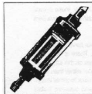
Figure #9 - Purolator makes an excellent filter with a replaceable screen. This type of filter must be safety wired to prevent thumb screw from vibrating down threaded shank. See text for more on this situation.
