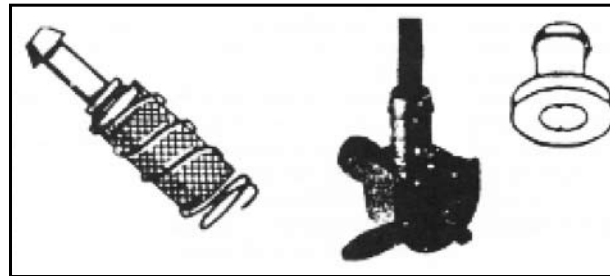
Figure #1 - Special attention must be paid to fuel tank pick ups. Here are two of the most common. On the left is a brass screen that slips onto the pick up line. On the right is a tank access fitting with shut off valve. This valve uses the grommet shown to seal the tank from one side only access.
