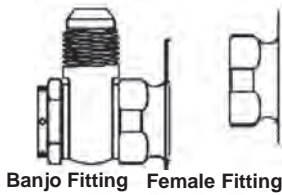
Banjo Fitting Female Fitting
